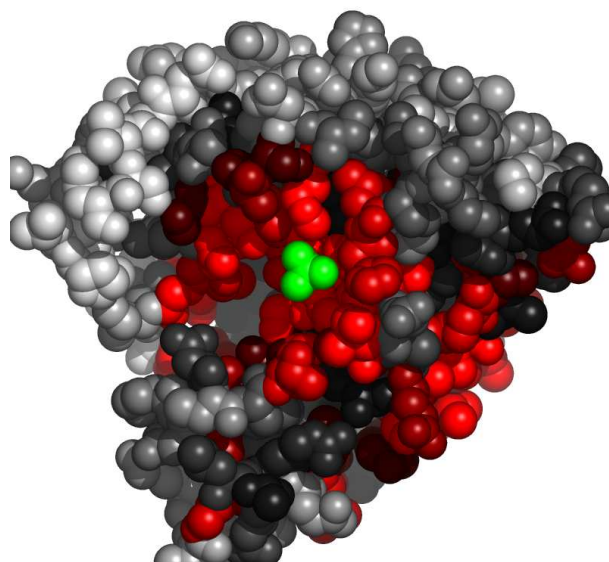
Fig. 5. Residues in 3dzvA, at the interface with sulfate ion, colored by their relative importance. The ligand (sulfate ion) is colored green. Atoms further than 30Å away from the geometric center of the ligand, as well as on the line of sight to the ligand were removed. (See Appendix for the coloring scheme for the protein chain 3dzvA.)
