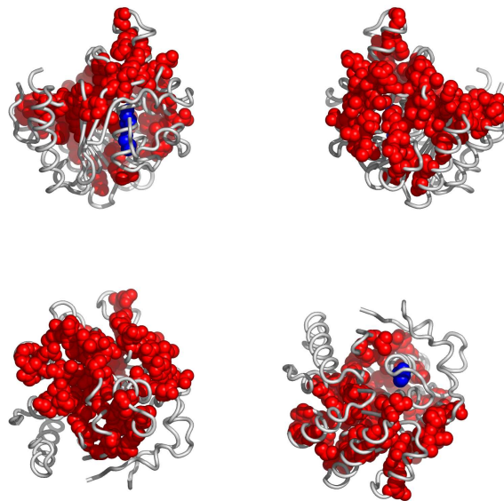
Fig. 4. Residues in 3dzvA, colored according to the cluster they belong to: red, followed by blue and yellow are the largest clusters (see Appendix for the coloring scheme). Clockwise: front, back, top and bottom views. The corresponding Pymol script is attached.
