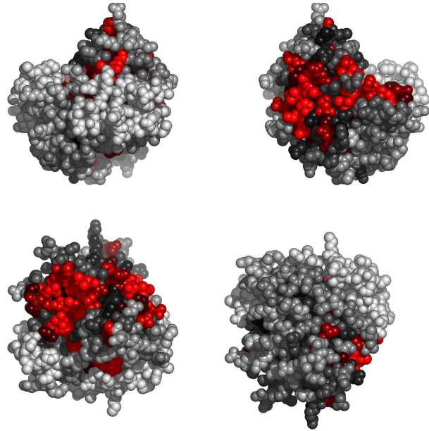
Fig. 3. Residues in 3dzvA, colored by their relative importance. Clockwise: front, back, top and bottom views.
