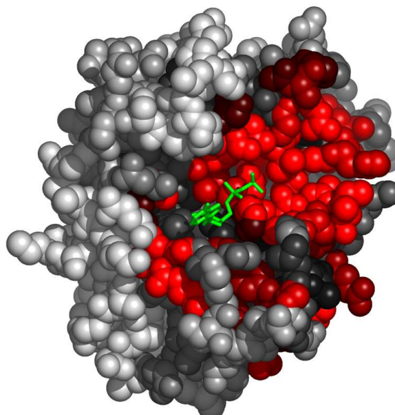
Fig. 6. Residues in 3dzvA, at the interface with ADP, colored by their relative importance. The ligand (ADP) is colored green. Atoms further than 30Å away from the geometric center of the ligand, as well as on the line of sight to the ligand were removed. (See Appendix for the coloring scheme for the protein chain 3dzvA.)
