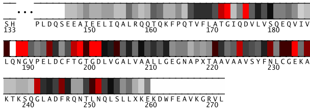
Fig. 2. Residues 133-272 in 3dzvA colored by their relative importance. (See Appendix, Fig.8, for the coloring scheme.)
