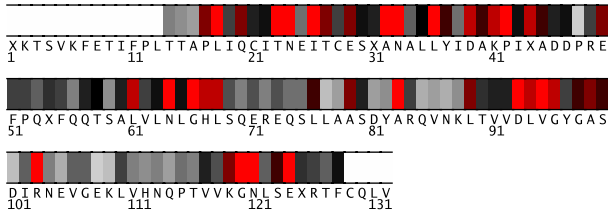
Fig. 1. Residues 1-132 in 3dzvA colored by their relative importance. (See Appendix, Fig.8, for the coloring scheme.)
