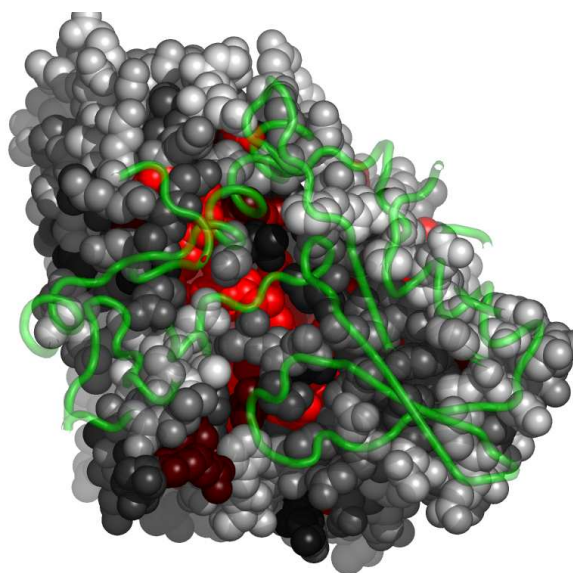
Fig. 7. Residues in 2fb2A, at the interface with 2fb2B, colored by their relative importance. 2fb2B is shown in backbone representation (See Appendix for the coloring scheme for the protein chain 2fb2A.)
