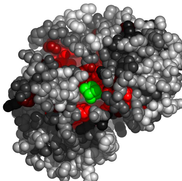
Fig. 9. Residues in 2fb2A, at the interface with iron/sulfur cluster, colored by their relative importance. The ligand (iron/sulfur cluster) is colored green. Atoms further than 30Å away from the geometric center of the ligand, as well as on the line of sight to the ligand were removed. (See Appendix for the coloring scheme for the protein chain 2fb2A.)
