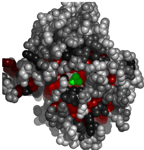
Fig. 8. Residues in 2fb2A, at the interface with sulfate ion, colored by their relative importance. The ligand (sulfate ion) is colored green. Atoms further than 30Å away from the geometric center of the ligand, as well as on the line of sight to the ligand were removed. (See Appendix for the coloring scheme for the protein chain 2fb2A.)
