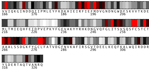
Fig. 2. Residues 166-329 in 2fb2A colored by their relative importance. (See Appendix, Fig.10, for the coloring scheme.)
