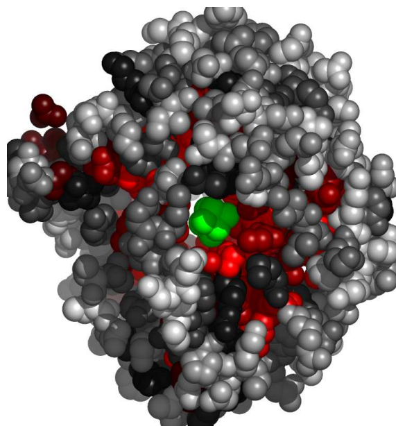
Fig. 6. Residues in 2fb2A, at the interface with iron/sulfur cluster, colored by their relative importance. The ligand (iron/sulfur cluster) is colored green. Atoms further than 30Å away from the geometric center of the ligand, as well as on the line of sight to the ligand were removed. (See Appendix for the coloring scheme for the protein chain 2fb2A.)
