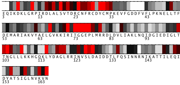
Fig. 1. Residues 3-165 in 2fb2A colored by their relative importance. (See Appendix, Fig.10, for the coloring scheme.)
