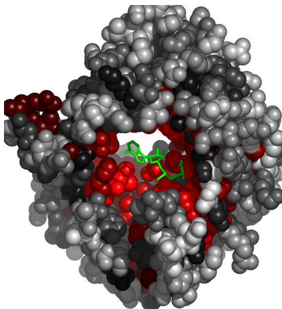
Fig. 5. Residues in 2fb2A, at the interface with s-adenosylmethionine, colored by their relative importance. The ligand (s-adenosylmethionine) is colored green. Atoms further than 30 Å away from the geometric center of the ligand, as well as on the line of sight to the ligand were removed. (See Appendix for the coloring scheme for the protein chain 2fb2A.)
