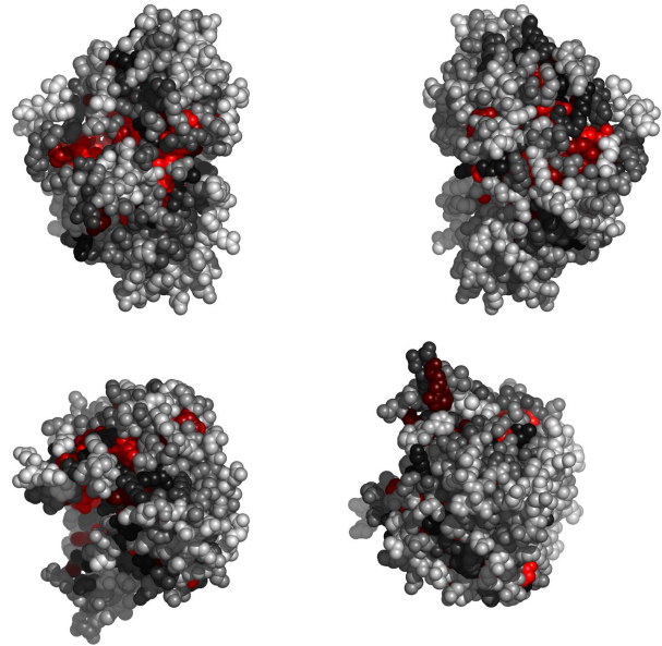
Fig. 3. Residues in 2fb2A, colored by their relative importance. Clockwise: front, back, top and bottom views.
